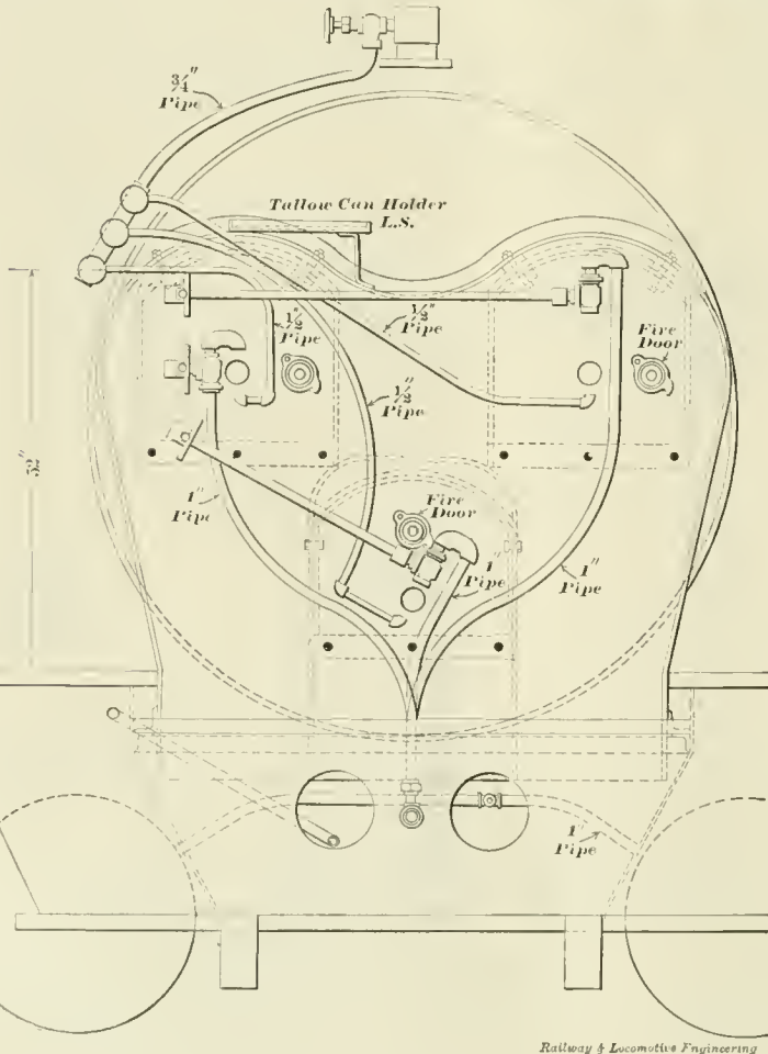
PLAYER-VAUCLAIN OIL-BURNING COMPOUND.
